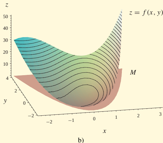
Obr. 6.3: f: z = 2x^3 + 4x^2 + y^2 - 2xy, x^2 - 2 \leq y \leq 4
