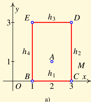
Obr. 6.2: f: z = x^2 + 4xy - 8x - 8y + 20 , 1 \leq x \leq 3 , 0 \leq y \leq 3
