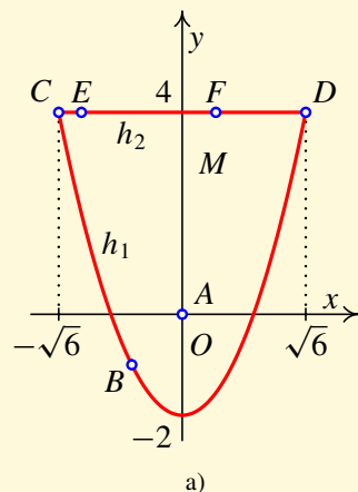
Obr. 6.3: f: z = 2x^3 + 4x^2 + y^2 - 2xy, x^2 - 2 \leq y \leq 4
