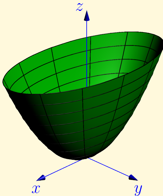
Obr. 8.4: Eliptický paraboloid((8.12): a = 4 , b = 2 , c = 1 )
