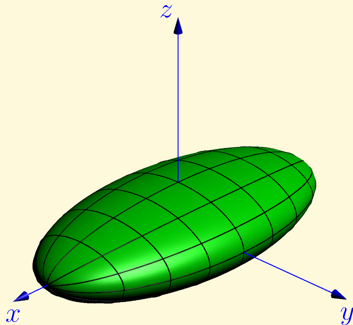
Obr. 8.3: Trojosý elipsoid((8.11): a = 4 , b = 2 , c = 1 )
