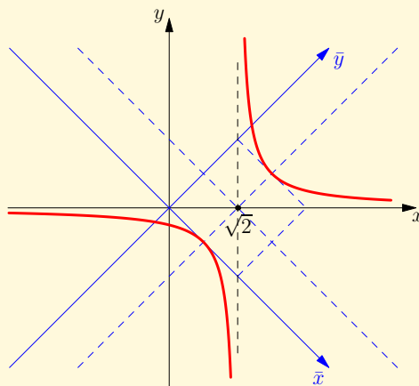
Obr. 7.13: Rovnoosá hyperbola 2xy - 2\sqrt{2}y = 1
