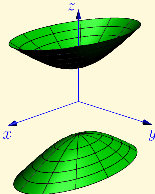
Obr. 8.6: Dvojdílný hyperboloid((8.14): a = 4 , b = 2 , c = 1 )
