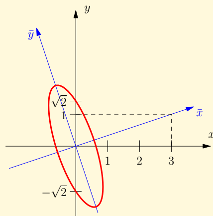
Obr. 7.14: Elipsa 10x^2 + 6xy + 2y^2 = 4
