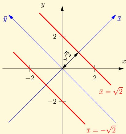
Obr. 7.12: Degenerovaná parabola x^2 + 2xy + y^2 = 4
