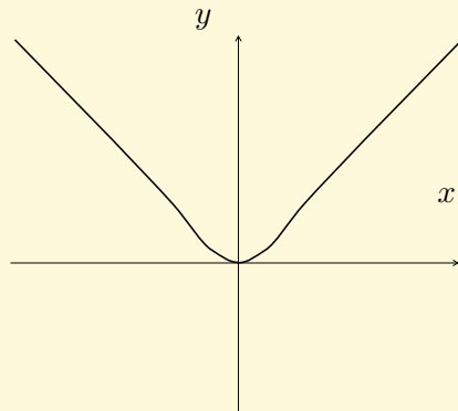
Obr. 15.6: Graf f(x) = (x^2 + \varepsilon)^{\frac{1}{2}}
